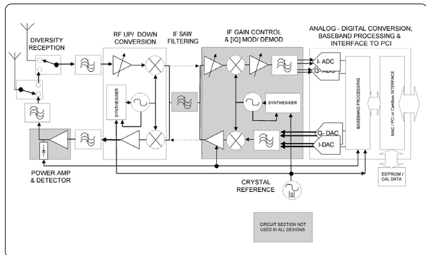
Figure 2: Block diagram of a WLAN card
