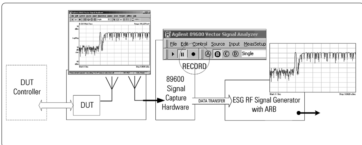
Figure 24: Signal record/replay of suspect signal using Agilent 89600 Vector Signal Analyzer and ESG
