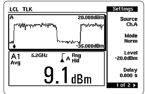
Figure 9: Average power measurement of IEEE 802.11a, using EPM-P
