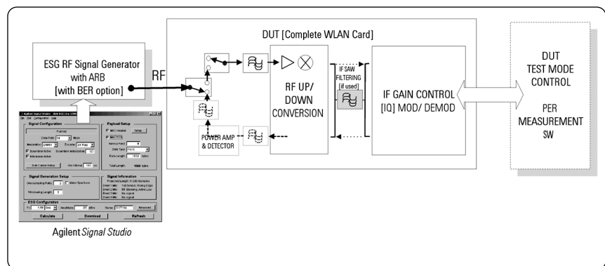
Figure 28: Diagram of complete receiver measurement path
