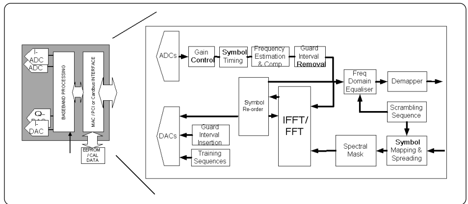
Figure 3: Digital processing blocks for an OFDM transceiver
