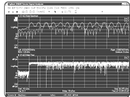
Figure 19b: Frequency change during frame
